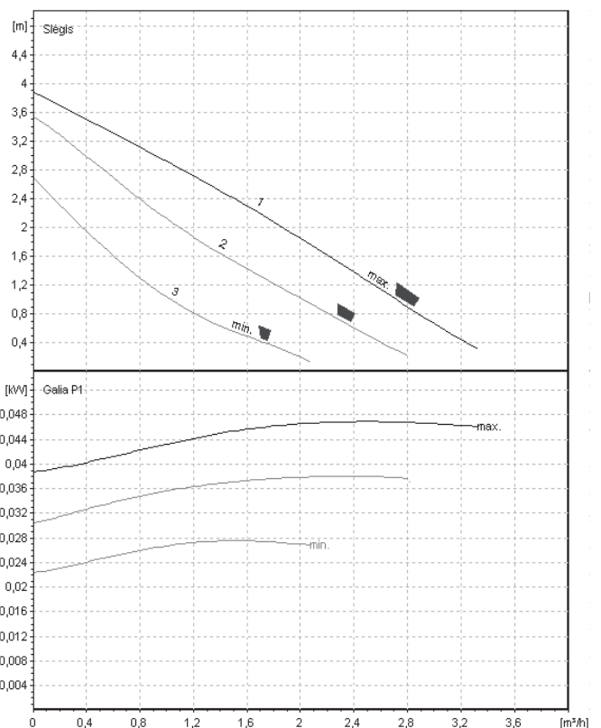
Wilo Star-RS 25/4
