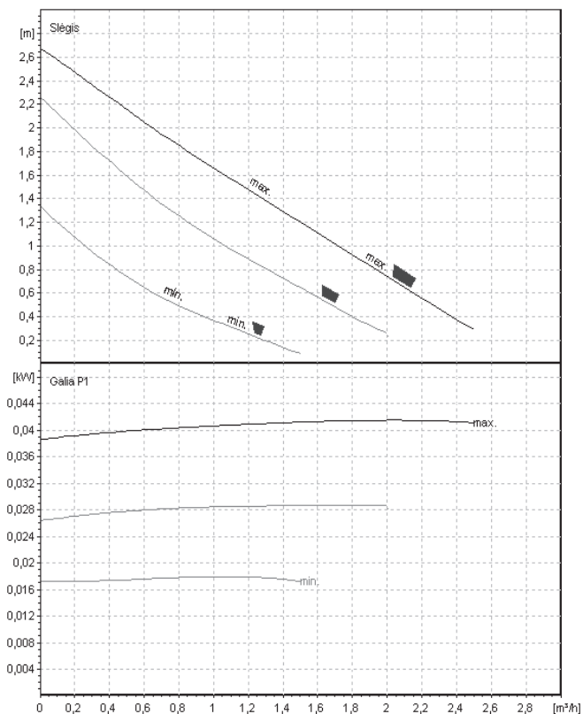
Wilo Star-RS 25/2
